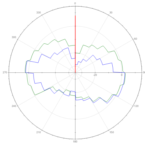
E-Plane Pattern
