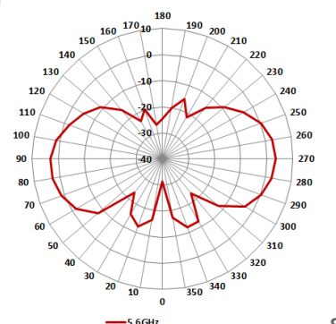
External Antenna E-Plane Pattern
