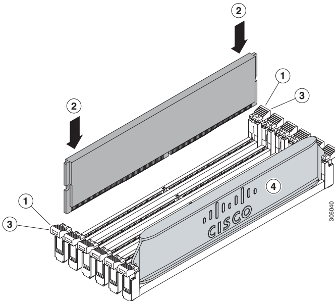
Figure 13 Replacing Memory
