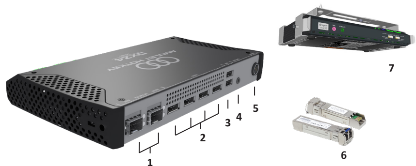
DXZ4-M rear view: 1 Network connections. 2 DisplayPort sockets. 3 USB ports. 4 Audio socket. 5 DC inlet. 6 SFP modules. 7 Under-desk bracket (optional).
