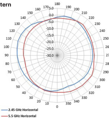
E-Plane Pattern
