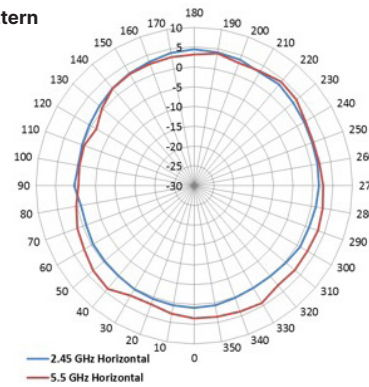
E-Plane Pattern
