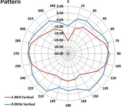
E-Plane Pattern
