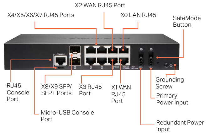
TZ570 Rear Panel
