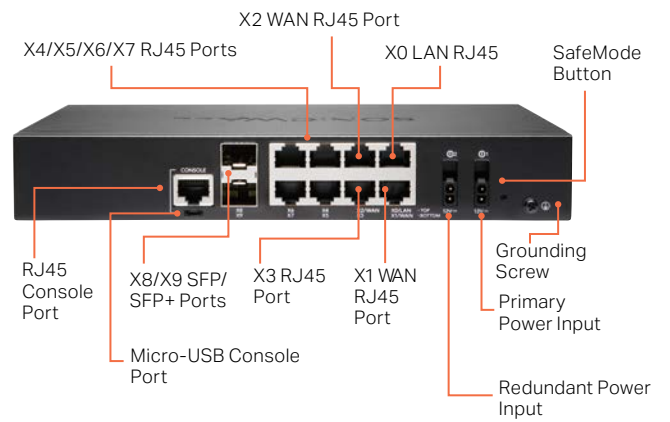
TZ670 Rear Panel
