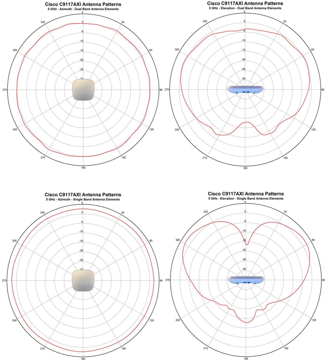
Figure 1. Antenna Radiation Patterns for C9117AXI
