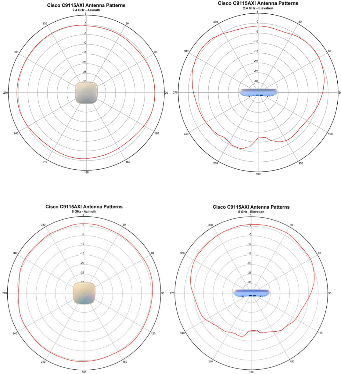
Figure 2. Antenna radiation pattern
