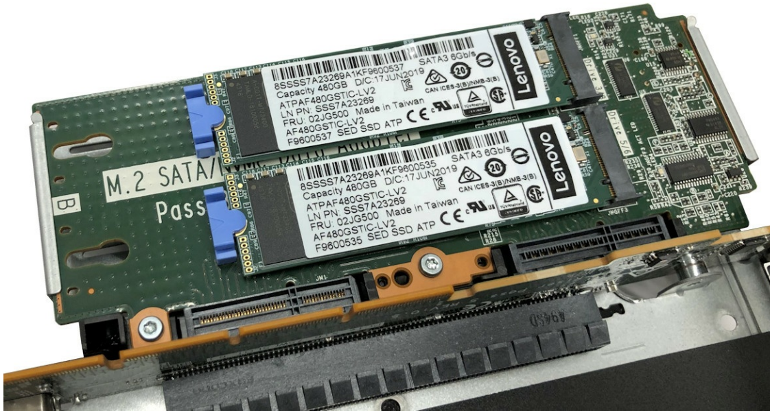
Figure 5. ThinkSystem SE350 M.2 SATA/NVMe 4-bay Data Drive Enablement Kit
