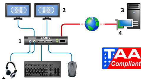
Example PCoIP system with DXZC-C. 1 DXZC-C. 2 Dual monitors. 3 Remote computer. 4 PCoIP host
