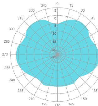
5 GHz Vertical
