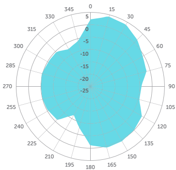
5 GHz Vertical
