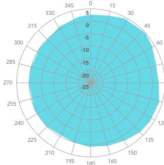
5 GHz Vertical
