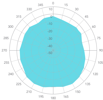
5 GHz Vertical
