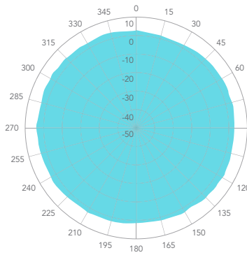
5 GHz Vertical
