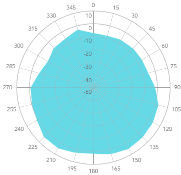
5 GHz Vertical
