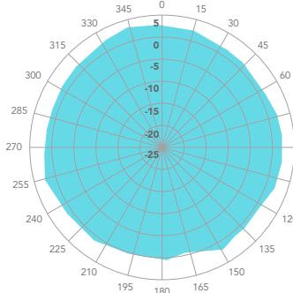
5 GHz Vertical
