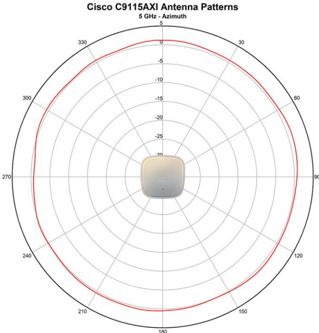
Figure 1. Antenna Radiation Pattern
