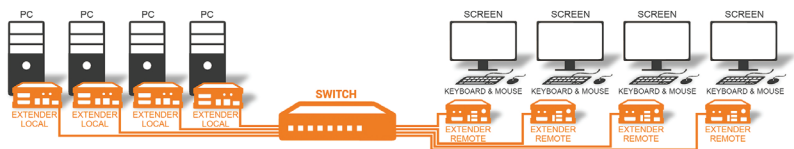
SWITCHING SYSTEM
