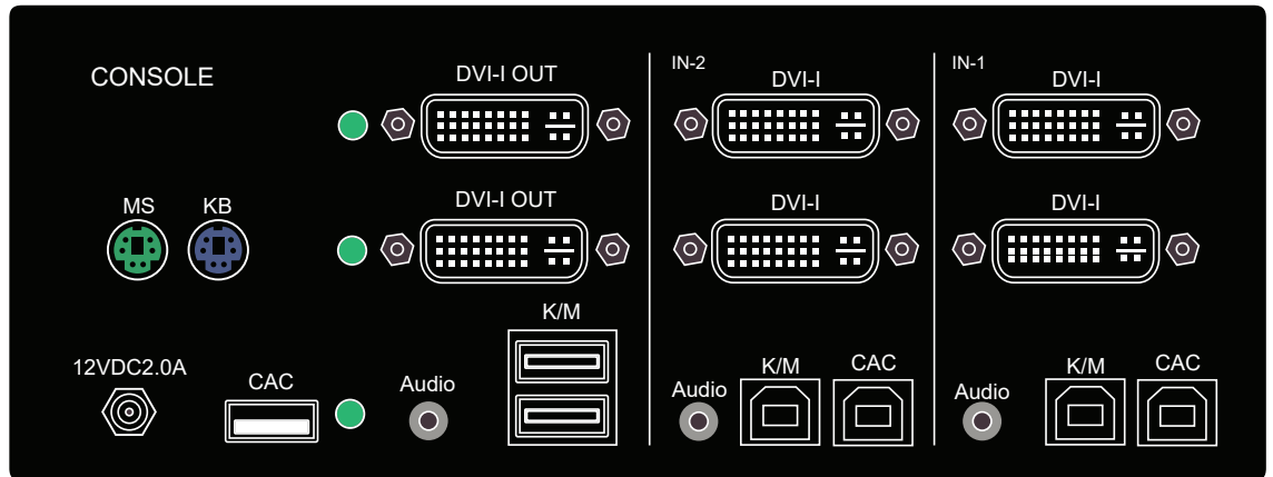
SS2P-DH-DVI-UCAC (Back)
