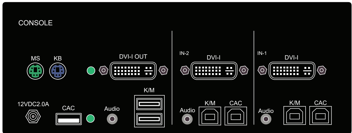
SS2P-SH-DVI-UCAC (Back)
