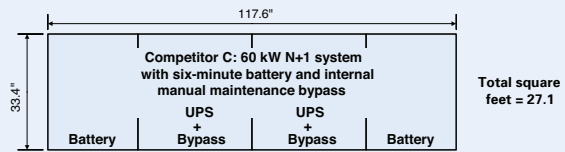
BladeUPS system footprint compared to competitors' footprints for 60 kW N+1 redundant application
