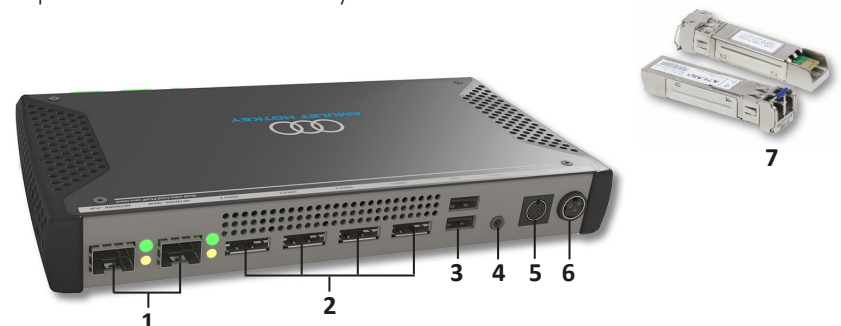
DXZ4-M rear view. 1 Network connections. 2 DisplayPort sockets. 3 USB ports. 4 Audio socket. 5 Feature connector. 6 DC inlet. 7 SFP modules.
