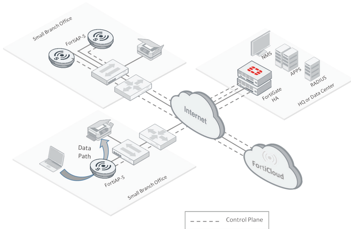
Cloud-managed and FortiGate-managed FAP-S series at remote sites
