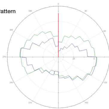
E-Plane Pattern
