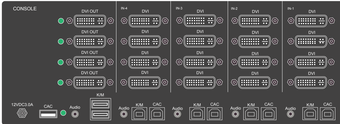
SDVN-4Q-P Back
