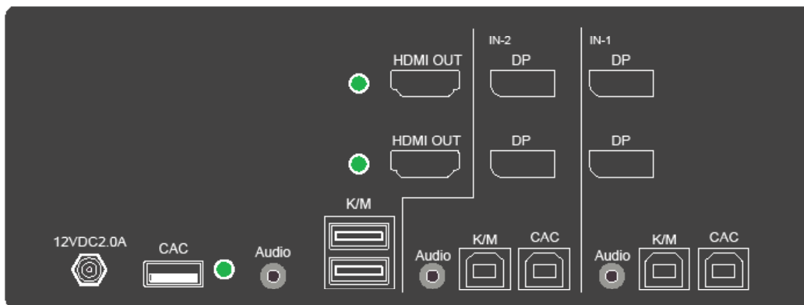
SDHN-2D-P Back
