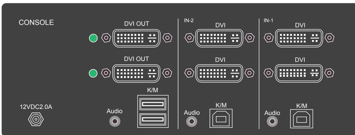
SDVN-2D Back
