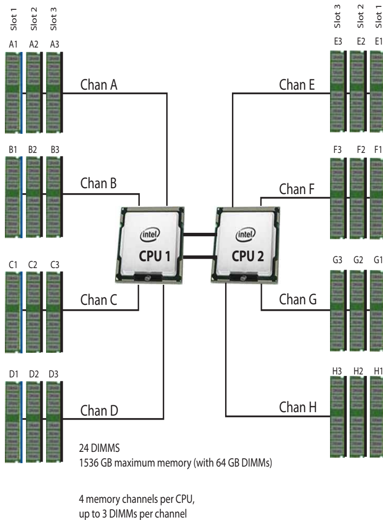
Figure 4 HX240c M4 Mode Memory Organization
