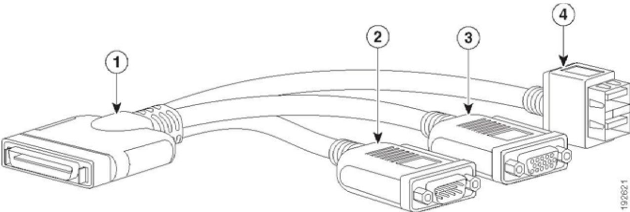
Figure 17 KVM Cable
