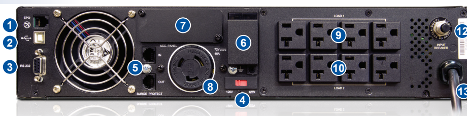
Rear View of E2000RTXL2U
