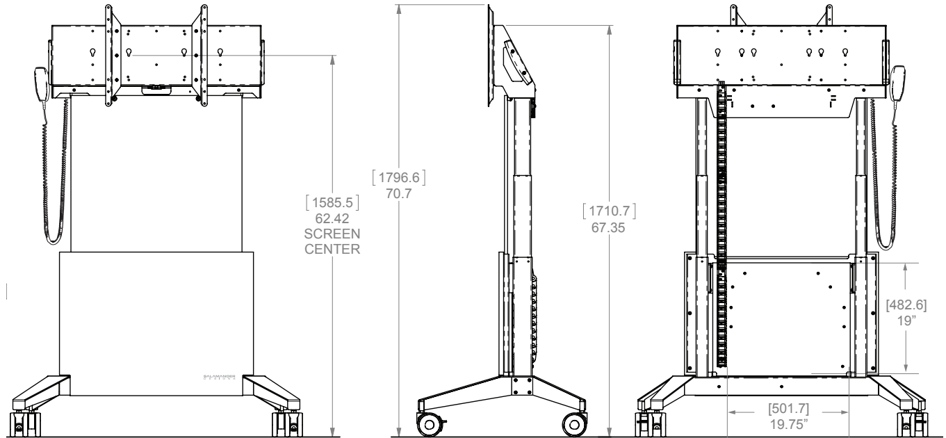
Equipment Mounting Panel
