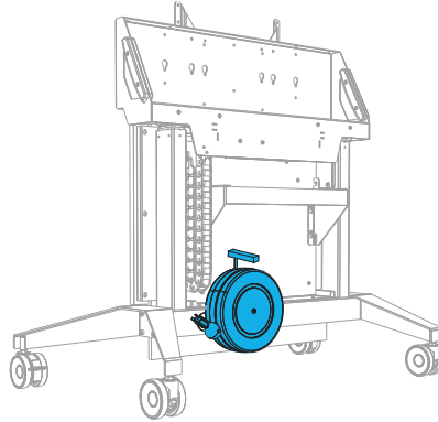
Cable Reel 30' Payout, 24" Tri-Tap Female End - FPSA/CR
