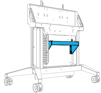
19" Rack Mounting 3 RU RM/VR/3U
