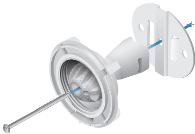
Installation Using the NanoBeamM Wall Mount Kit
