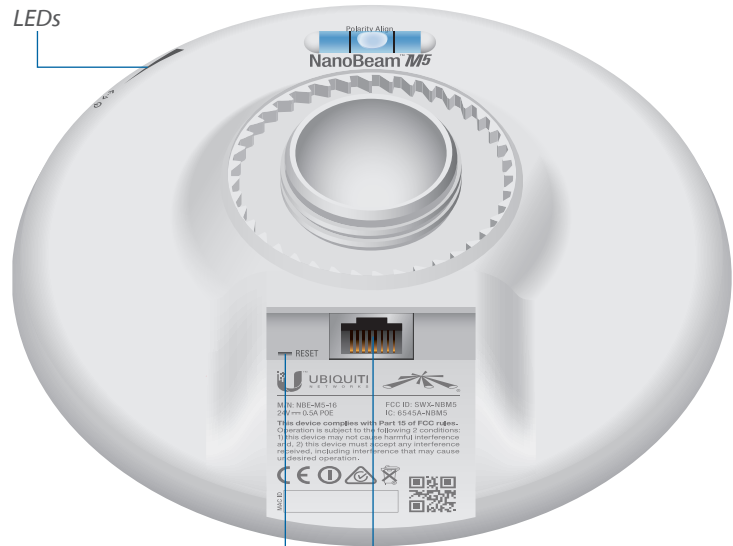
Reset Button
