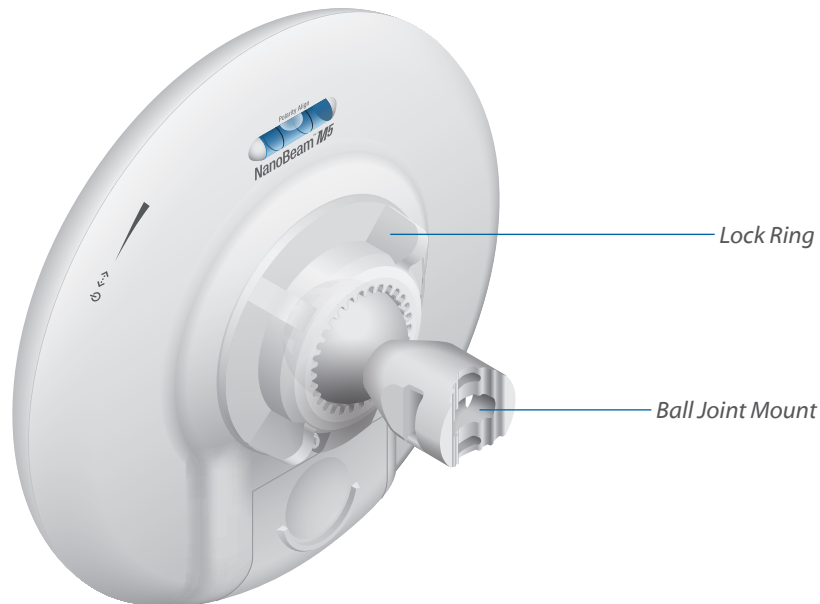
NBE-M5-16 with Mounting Hardware
