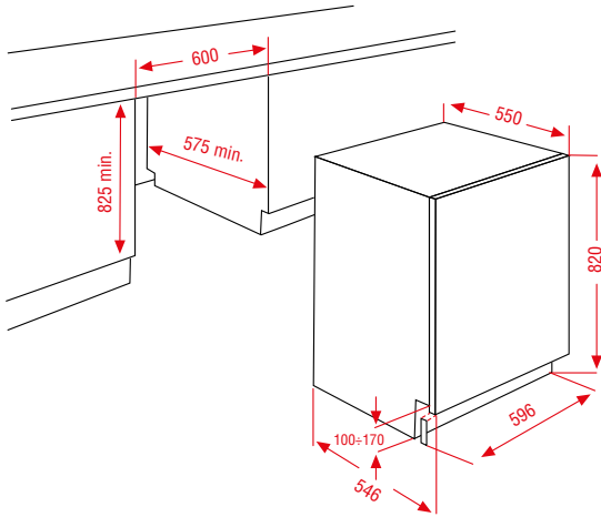
BUILT-IN WASHING MACHINE WMI 7462 W20
