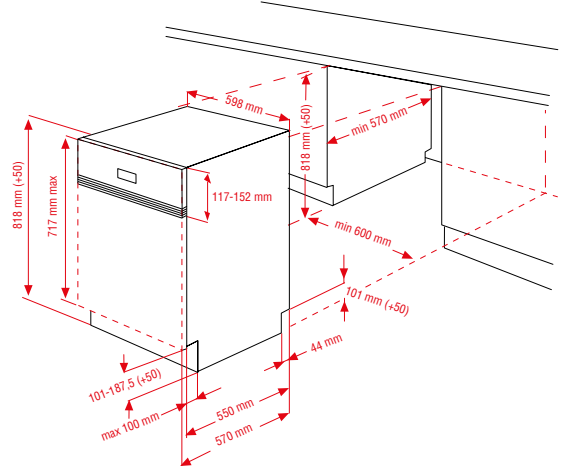
BUILT-IN DISHWASHER GVN 9483 E
