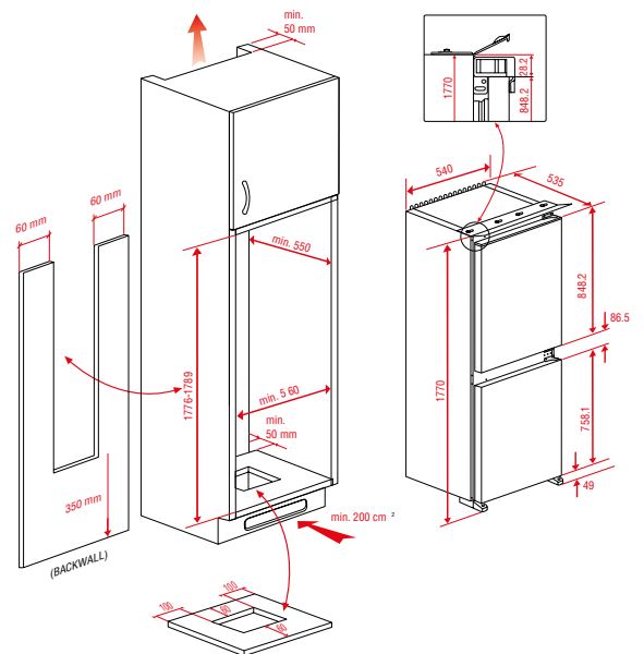
BUILT-IN REFRIGERATION KNM 1561 i
