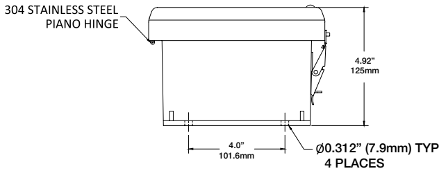
END VIEW
