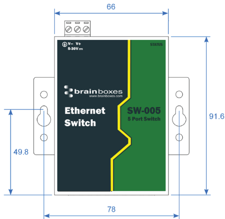
CASE DIMENSIONS - All dimensions in mm
