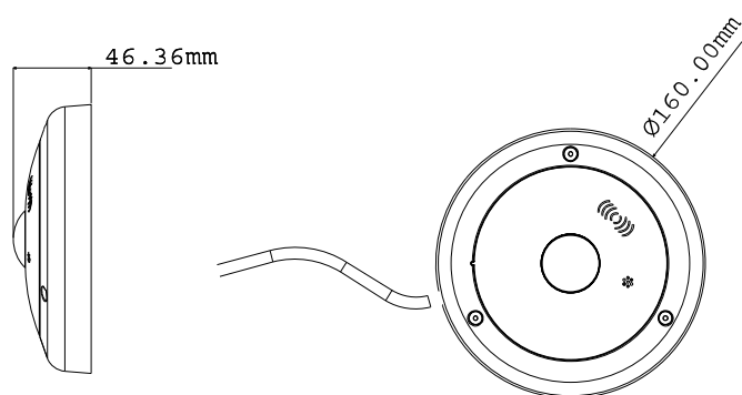
Hard-Ceiling Mount
