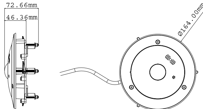
In-Ceiling Mount
