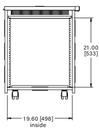
front view with door removed
