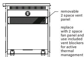
rear view
