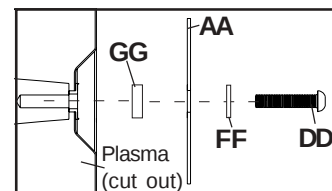
DETAIL 2
