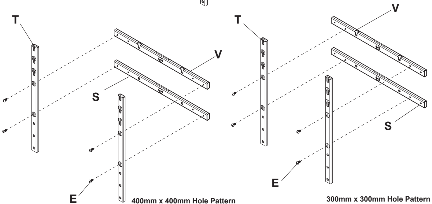
400mm x 400mm Hole Pattern
