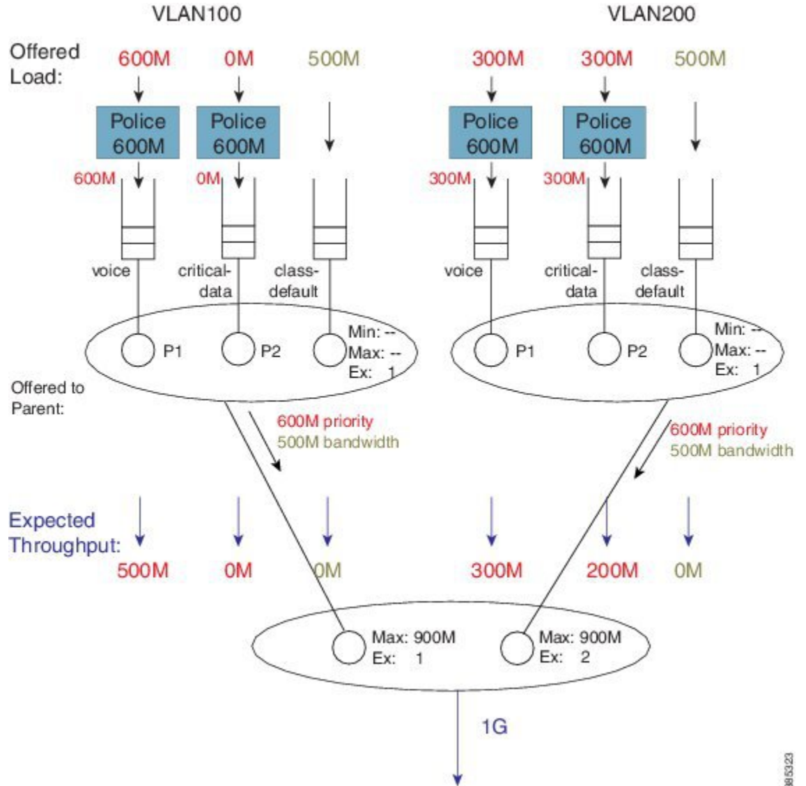
Figure 49: Child Schedule Apportions Bandwidth received from Parent Schedule
