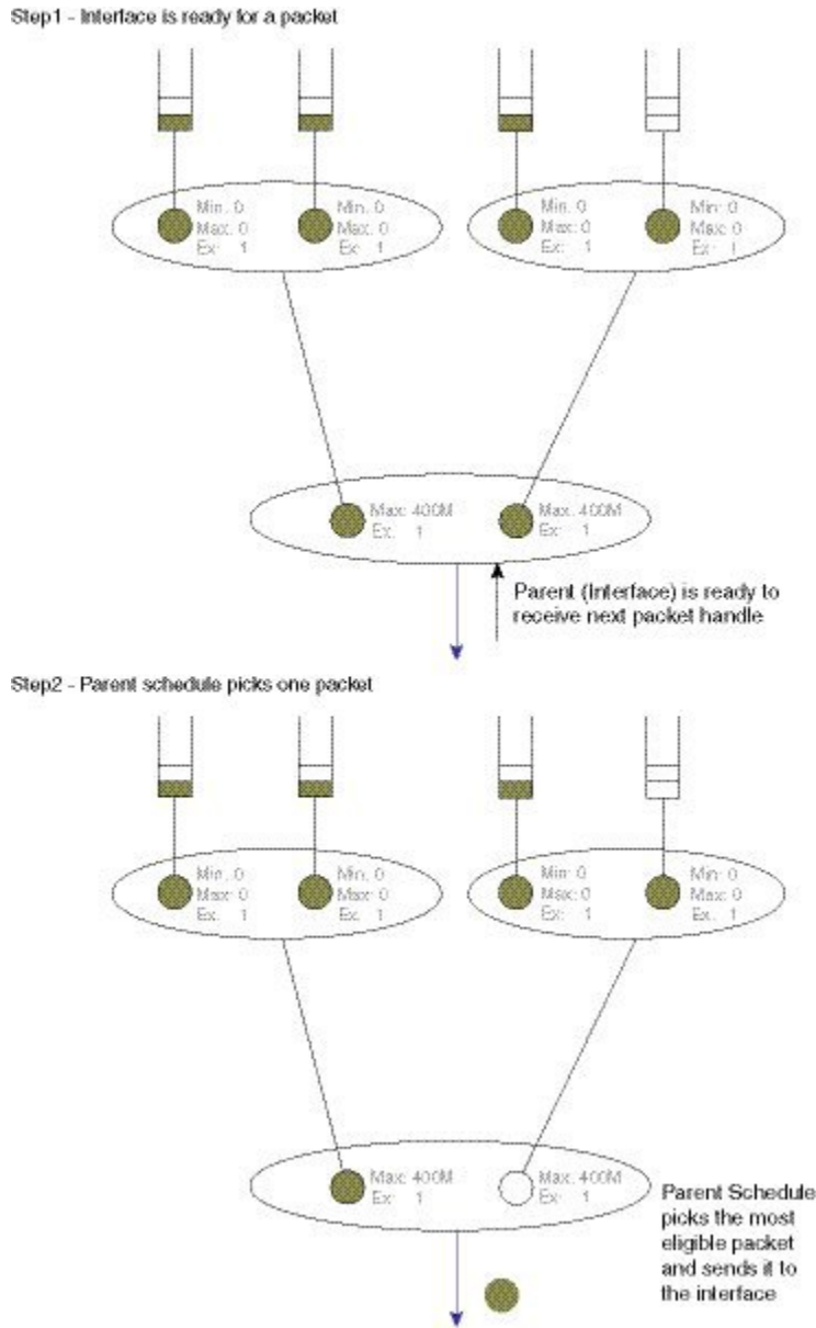
Figure 37: Scheduling Decision - Root to Leaf: Steps 1-2
