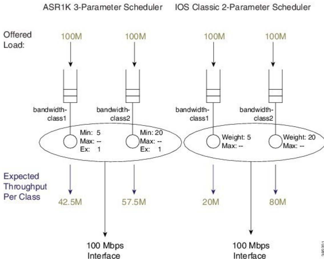
Figure 28: Same Configuration running on ASR 1000 with IOS XE and Router running IOS Classic
