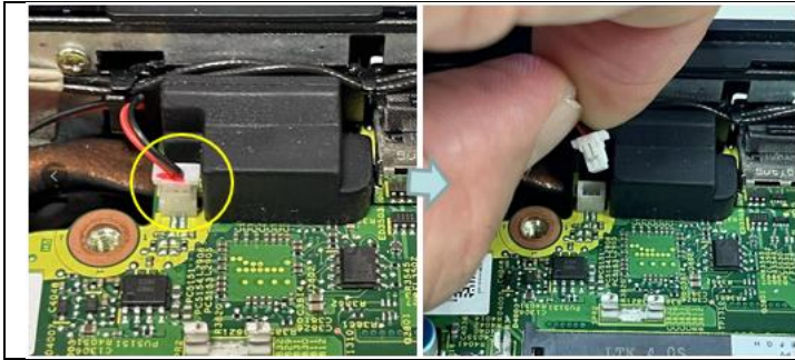
STEP 11. Remove speaker
