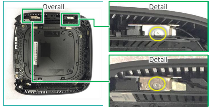
STEP 14. Unfasten "+" M2 screws
