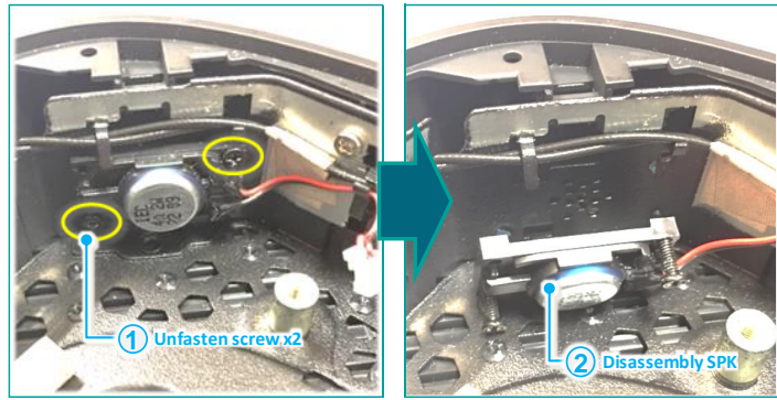
STEP 13. Unfasten "+" M3 screws and internal antenna
