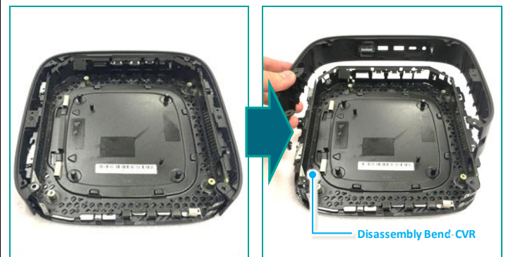
STEP 16. Remove Bend cover by hand
