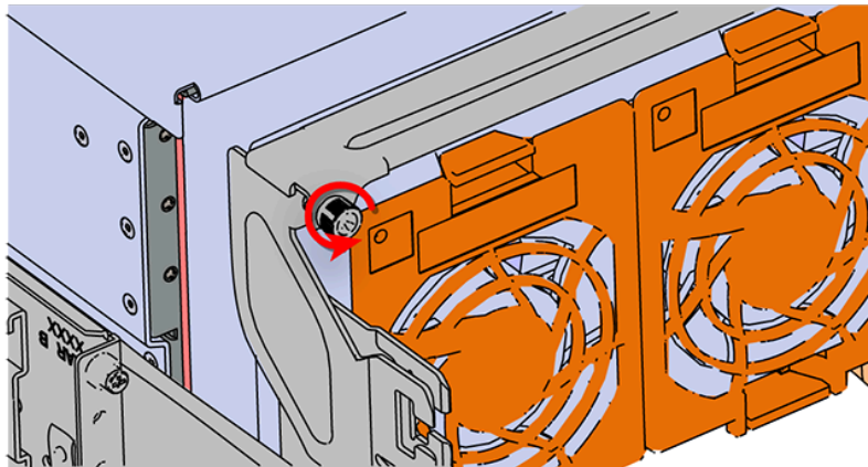
Figure 7: Unscrew Thumbscrew
