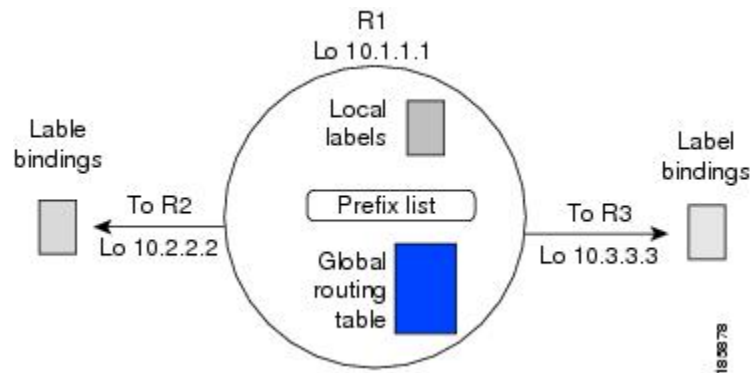
Figure 48: LDP Local Label Allocation Filtering Example
