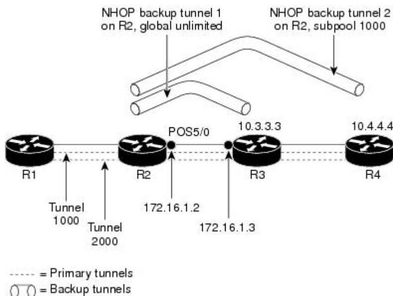
Figure 162: Backup Tunnels
