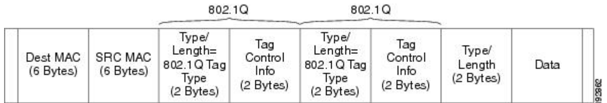
Figure 74: Ethernet VLAN QinQ Header
