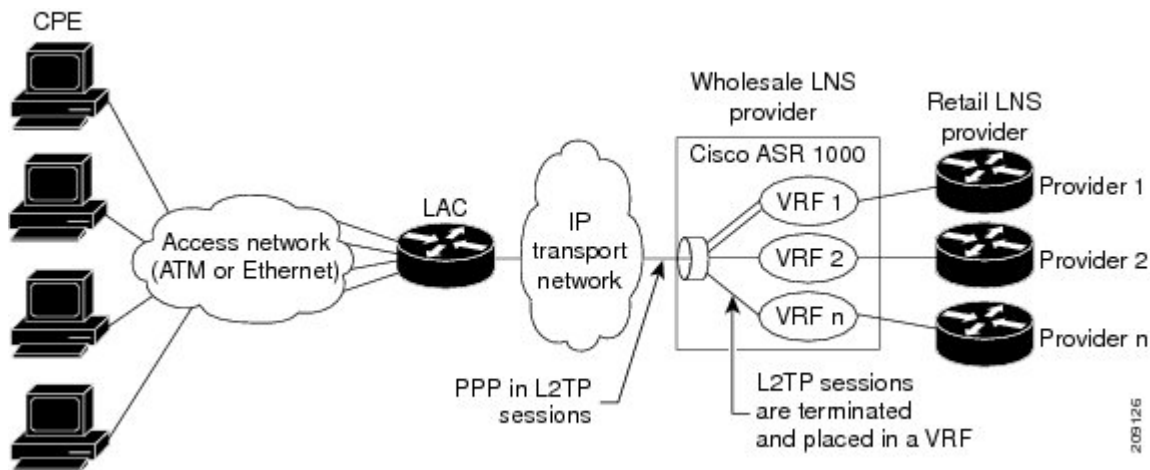
Figure 76: Terminating and Forwarding Sessions from the LAC
