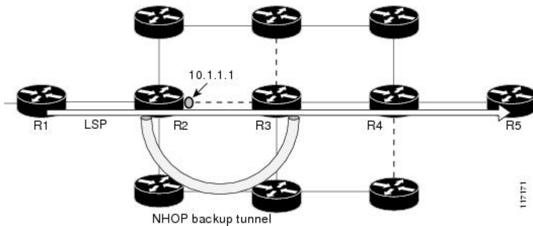
Figure 188: srlg exclude force--NHOP Autobackup Tunnel
