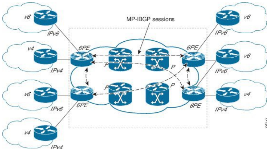
Figure 6: 6PE Device Topology
