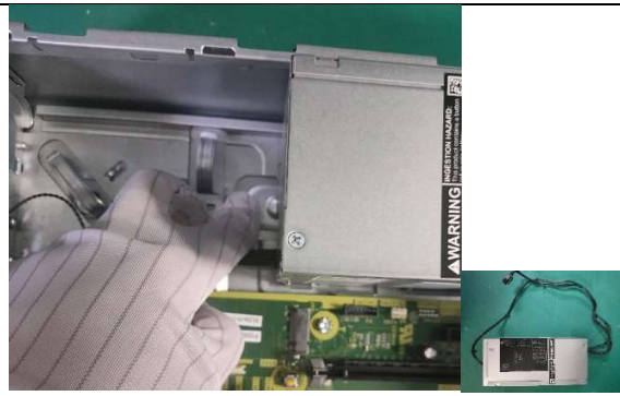
Step18 Remove speaker from Chassis.
