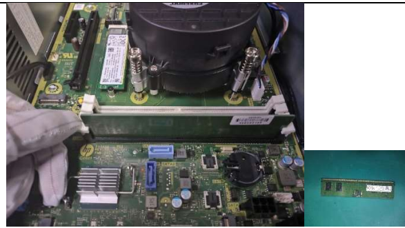
Memory PCB area surface is greater than 10 sq cm.
