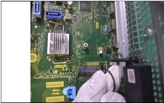
Step19 Loose the screws from the Motherboard.
