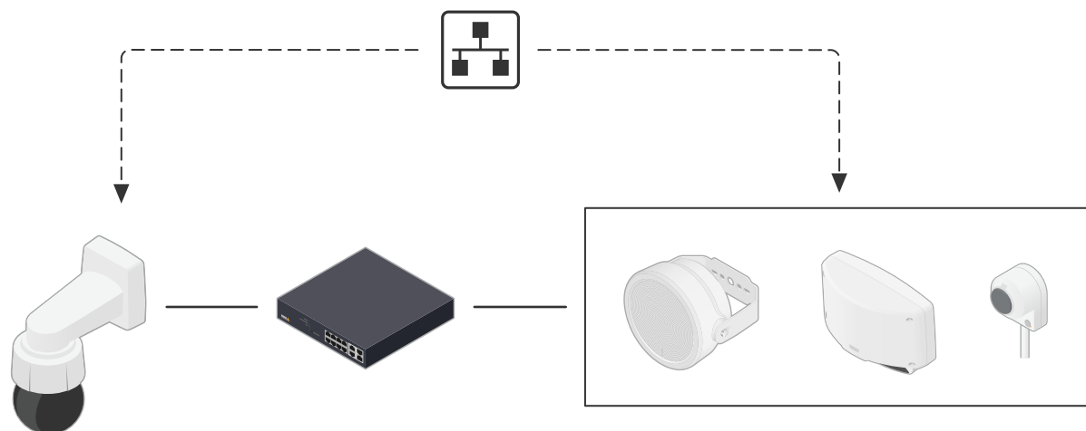
Figure 1. Edge-to-edge technology enables an Axis camera to pair with another Axis device, typically a speaker, radar, or microphone, to obtain seemingly camera-integrated features from that device.
