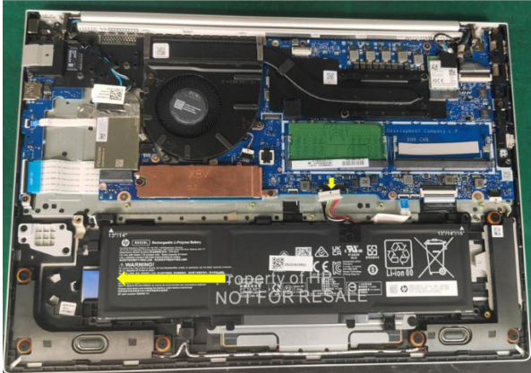
3.23 Use screwdriver to release main board #1 screw 9PCS
