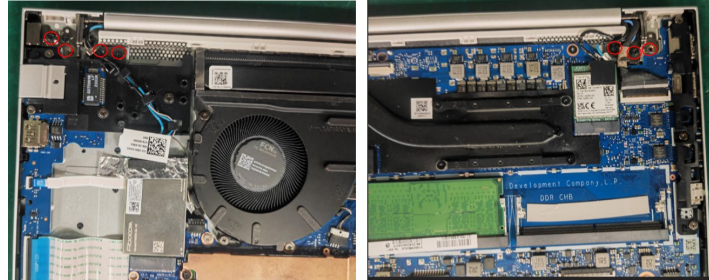
3.25 release hinge screw with screwdriver
