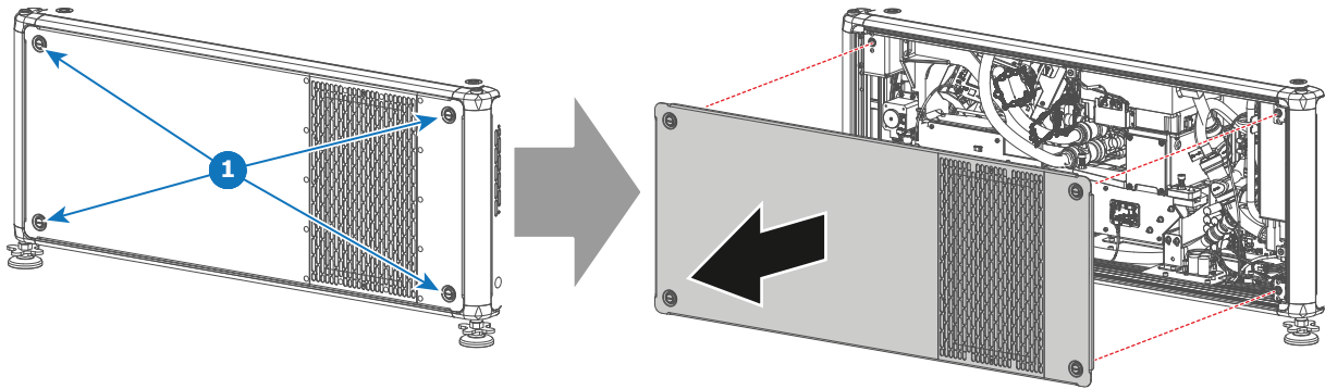
Image 9–2 Removal of the left cover (light processor side)
