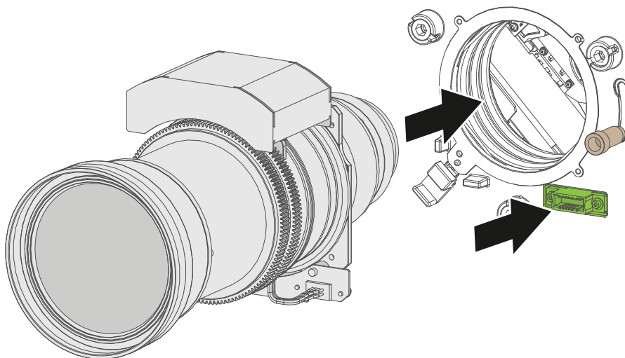
Image 5–3 Lens installation
