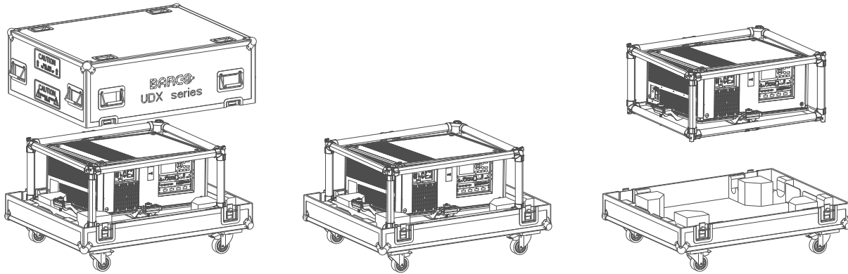
Image 7-1 UDX Flight case
