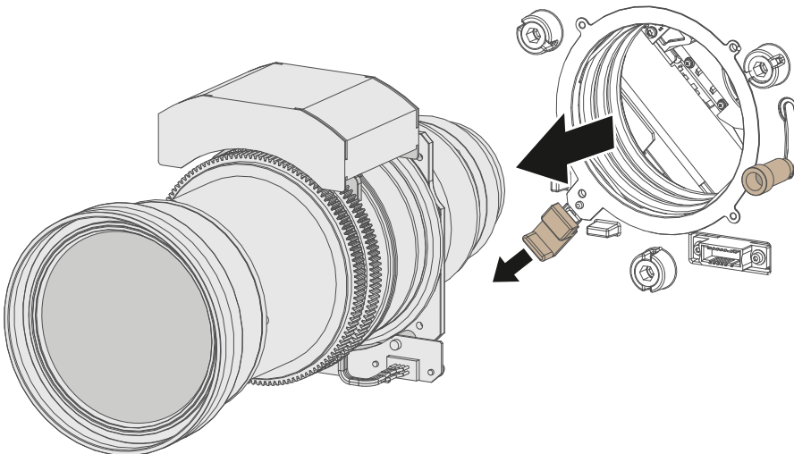
Image 5–16 Lens removal
