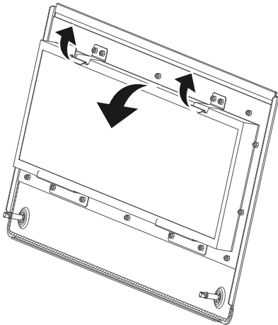
Image 6-2 Small top cover filter replacement
