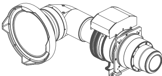
Image 5–19 Example of the 0.65 - 0.85:1 UST lens in both orientations
