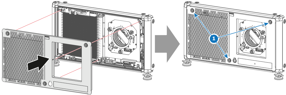
Image 9-6 Mount front cover
