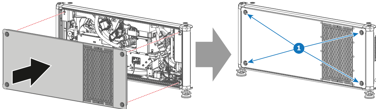
Image 9-7 Mount left cover (light processor side)
