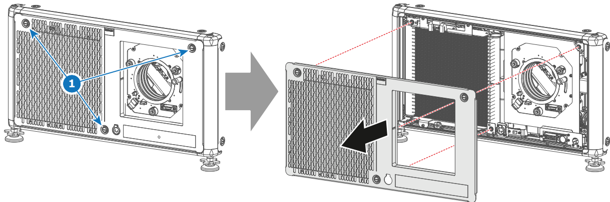
Image 9–1 Front cover removal
