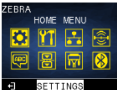
Figure 10 Home Menu
