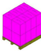
Carton: 490*295*518 mm 2*4 = 8 pcs/layer 8*2 layer = 16 pcs/pallet
