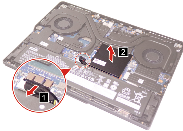
Figure 5. Remove the memory shielding
