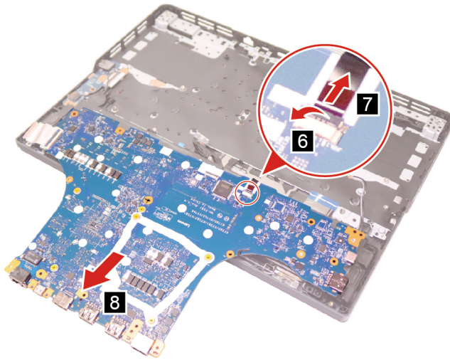
Figure 26. Disconnect the cable and then remove the system board
