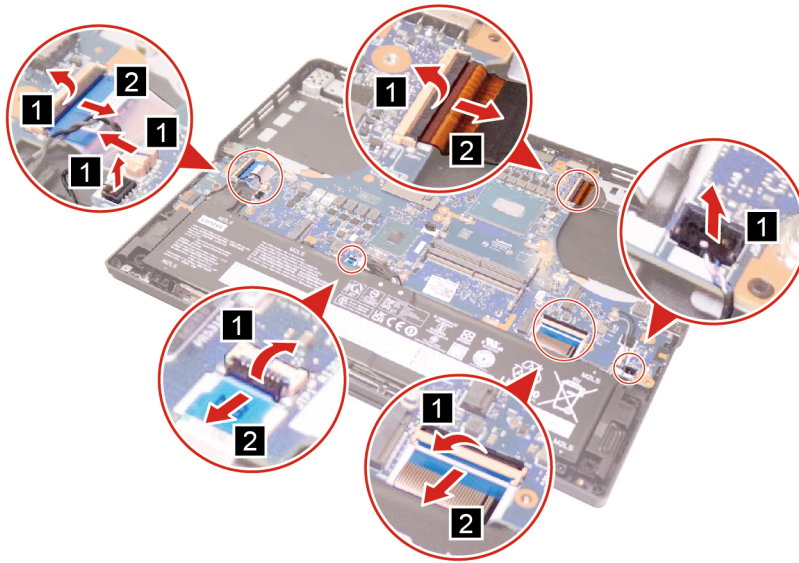
Figure 24. Disconnect cables
