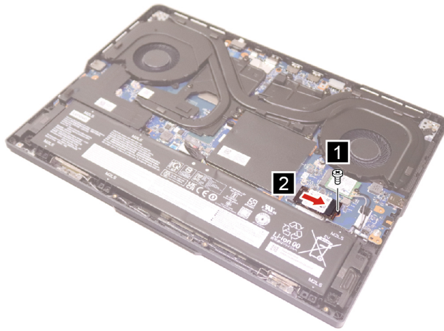
Figure 14. Remove the right 2242 SSD
