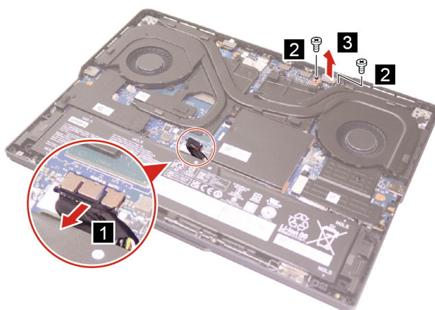
Figure 4. Remove the DC-in bracket
