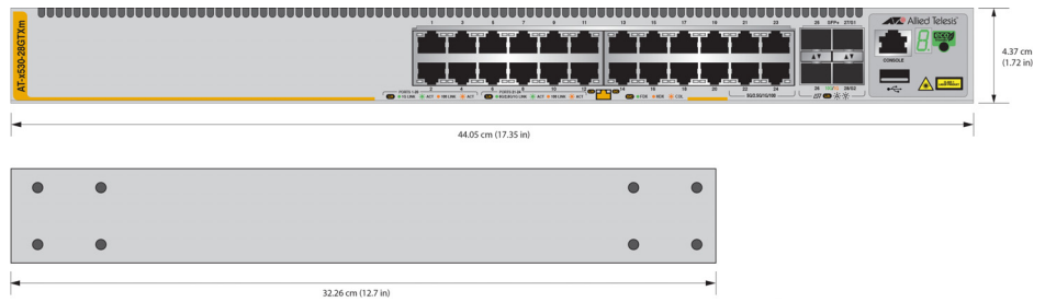
Figure 59. x530-28GTXm Dimensions
