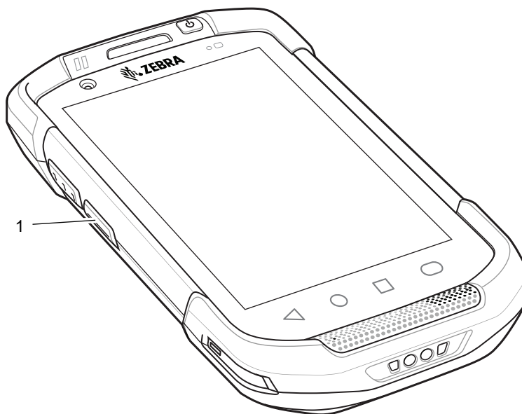
Figure 26 PTT Button
