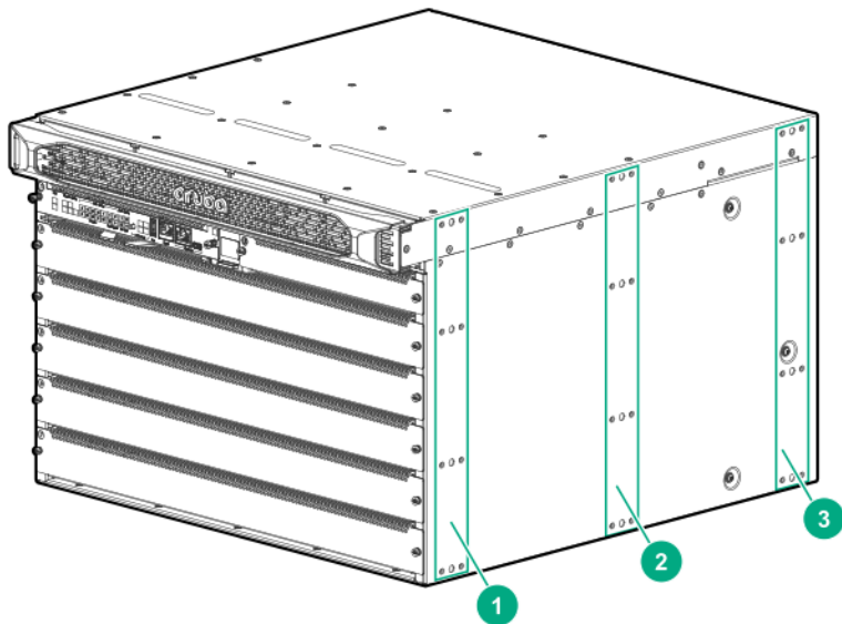
Figure 17 Two-post rack mount options
