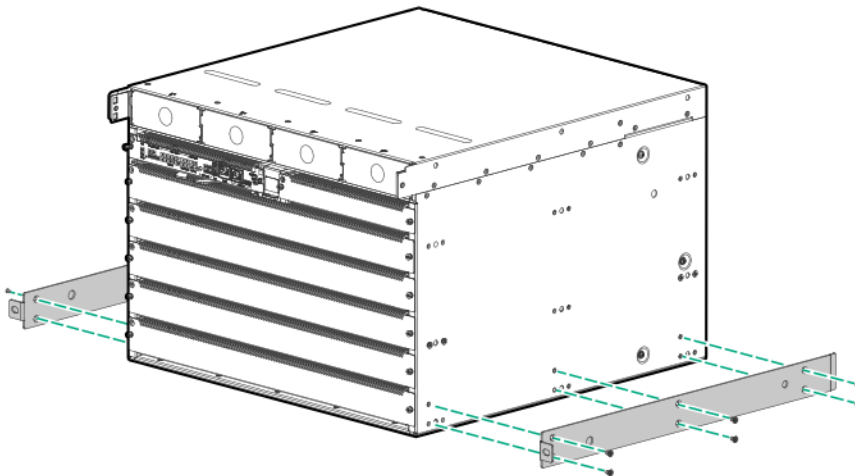
Figure 21 Attaching a rail spacer to each side of the chassis
