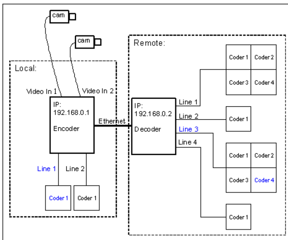
Figure 5.1: Encoder/Decoder connections
