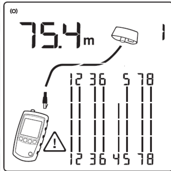
The MicroScanner™ display shows the length of the cable and an open on wire 4 at the far end.
