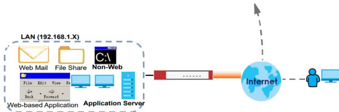
Figure 79 Network Access Mode: Split Tunnel Mode
