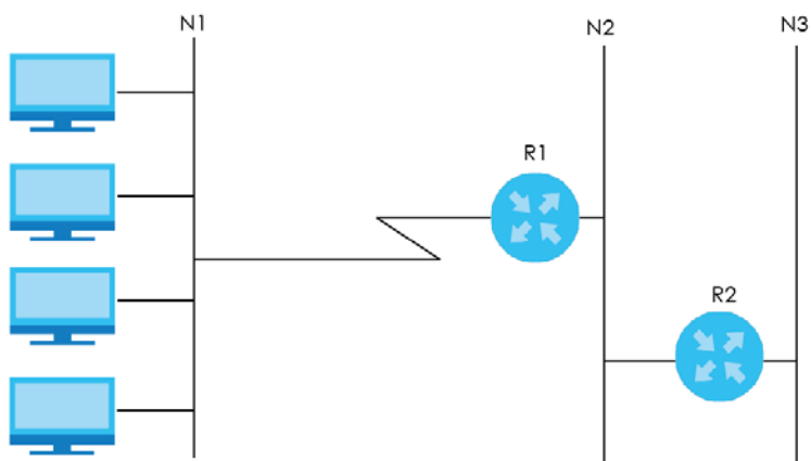
Figure 71 Example of Static Routing Topology
