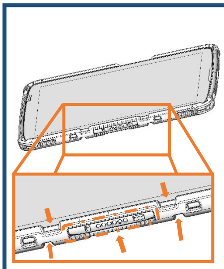
Alignment Sockets on the bottom of ZEBRA ET4X Tablet with Rugged Frame.
